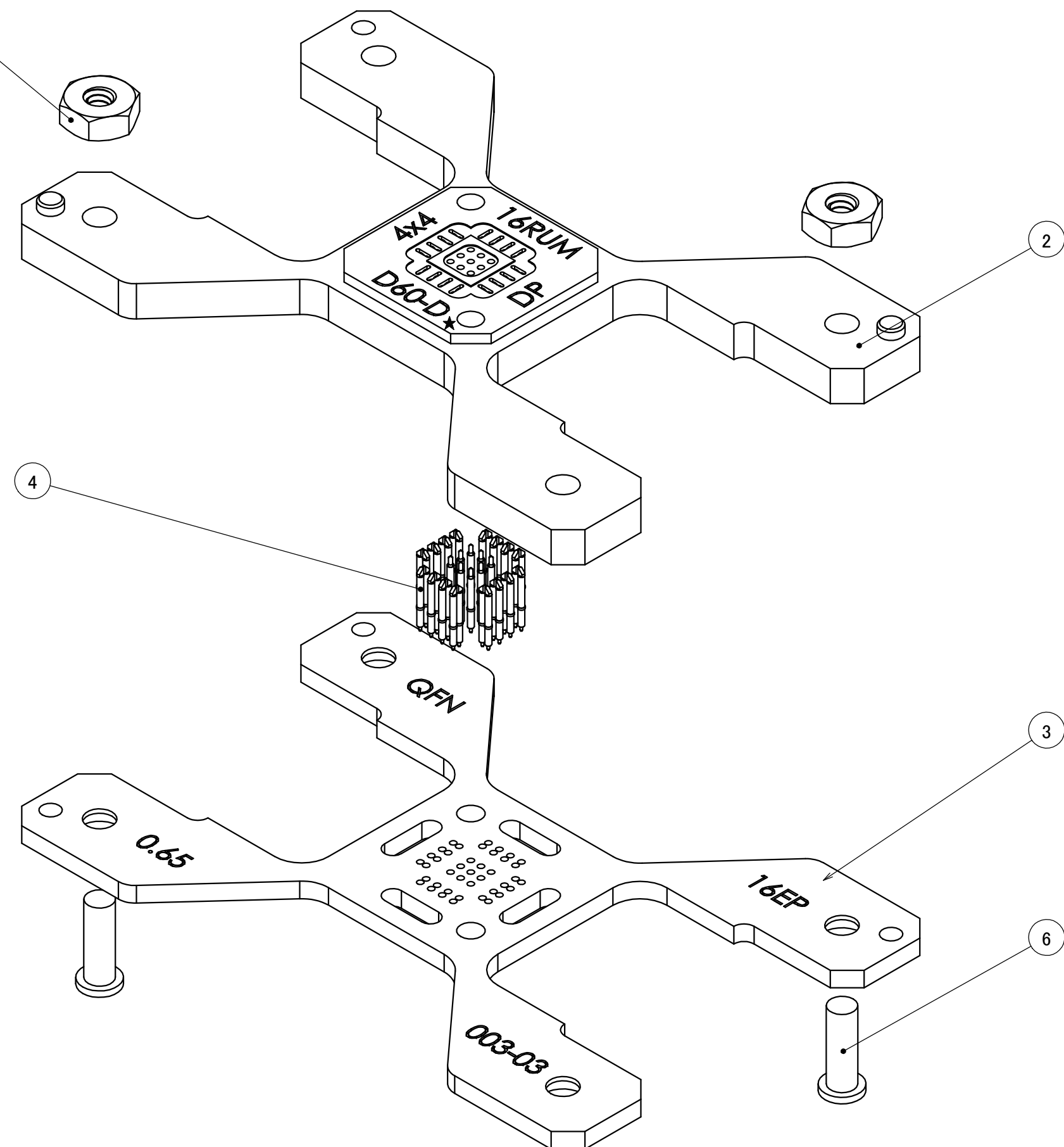
PIN BLOCK EXPLODED VIEW
