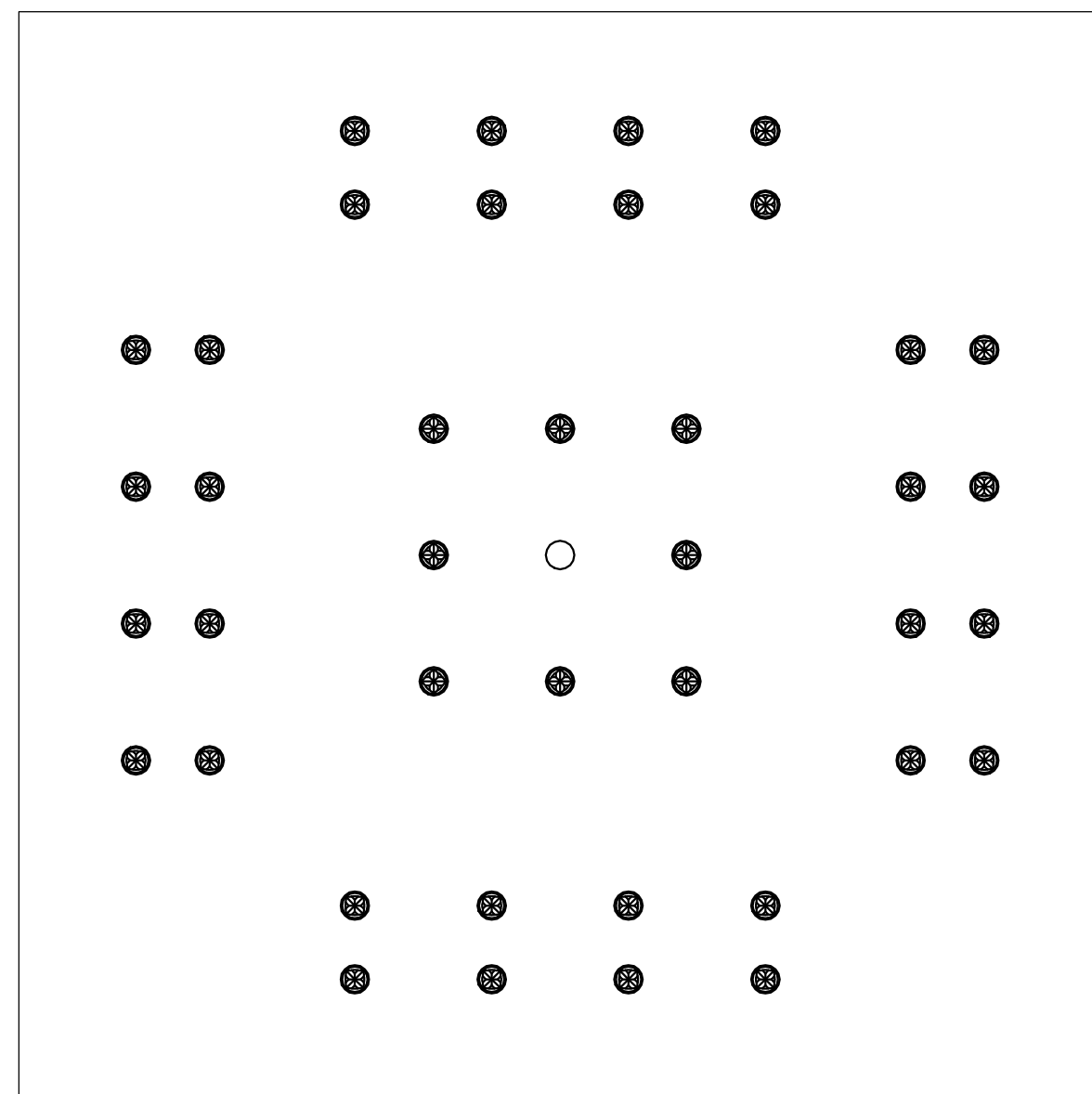
PIN MAP DETAIL FROM TOP VIEW SCALE=40:1
