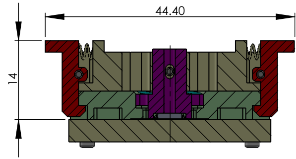
SECTION G-G SCALE 1.5 : 1
