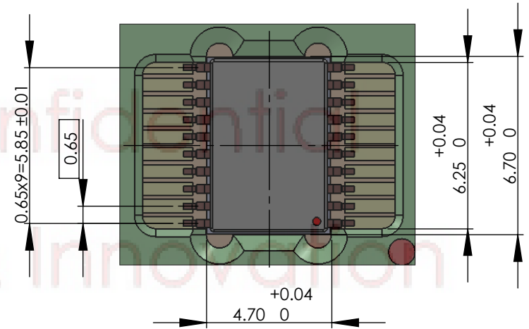
DETAIL H
